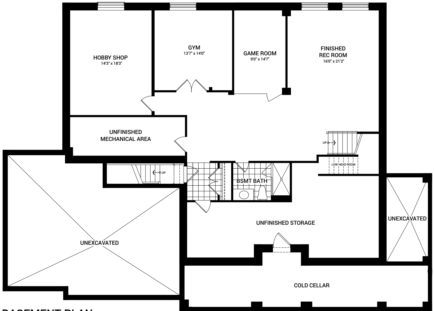
BASEMENT PLAN
